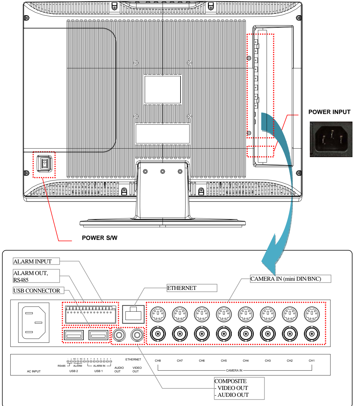
[Fig. 5-2 Rear & Side View]
